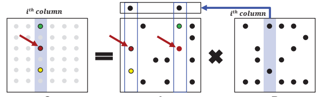
Fig. 4. Intra-Block Column-by-Column SpGEMM Algorithm
