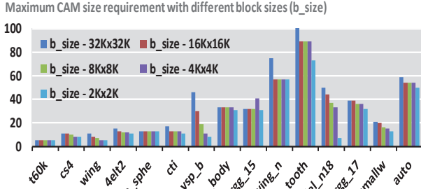
Fig. 8. CAM Size Evaluation.
