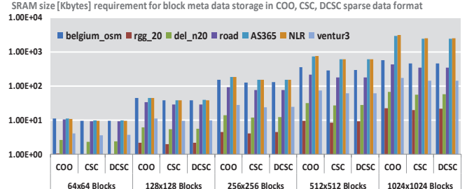
Fig. 11. Meta Data Storage Evaluation.
