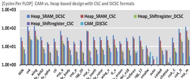
Fig. 10. CAM Performance Evaluation.
