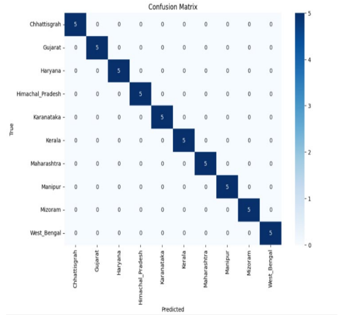
Fig. 6 Confusion matrix of tested data applying DenseNet121
