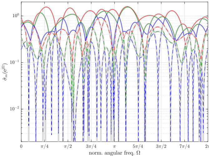
Fig. 8. Analytic singular values \hat{\sigma}_m(e^{j\Omega}) of the perturbed system \hat{A}(z) , with \sigma_{e,norm}^2 = 10^{-4} ; the moduli of \sigma_m(e^{j\Omega}) are underlaid in grey.
