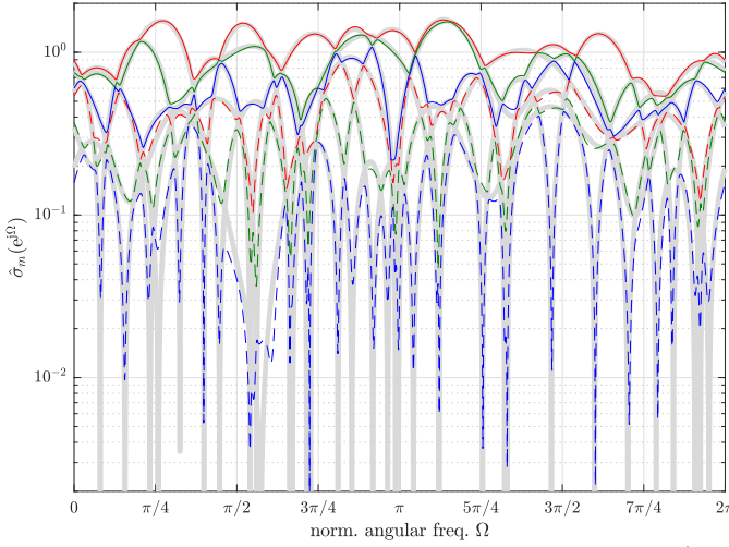
Fig. 7. Analytic singular values \hat{\sigma}_m(e^{j\Omega}) of the perturbed system \hat{A}(z) , with \sigma_{e,norm}^2 = 0.01 ; the moduli of \sigma_m(e^{j\Omega}) are underlaid in grey.
