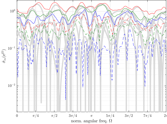
Fig. 6. Analytic singular values \hat{\sigma}_m(e^{j\Omega}) of the perturbed system \hat{A}(z) , with \sigma_{e,norm}^2 = 0.3 ; the moduli of \sigma_m(e^{j\Omega}) are underlaid in grey.
