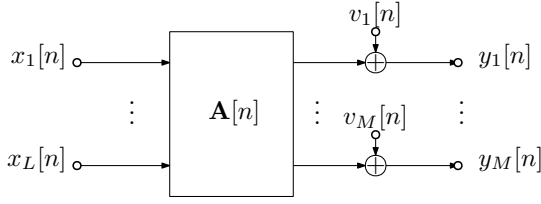
Fig. 2. System matrix \mathbf{A}[n] \longleftrightarrow \mathbf{A}(z) excited by inputs x_\ell[n] , \ell = 1, \dots, L source contributions and providing M outputs y_m[n] corrupted by additive noise v_m[n] , m = 1, \dots, M .
